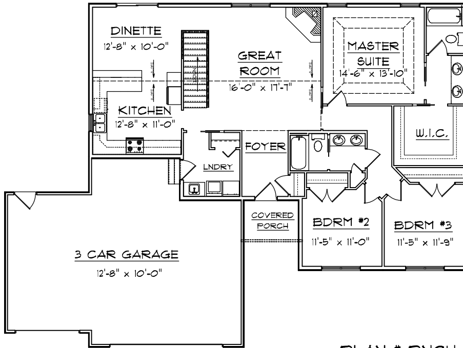
PLAN # RNCH-0111 1674 TOTAL SQFT 66'-0" WIDE X 49'-0" DEEP
