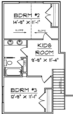
2ND FLOOR PLAN
